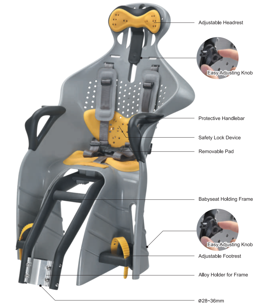
Install on Seat-tube
