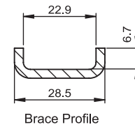
Brace Profile
