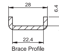
Brace Profile
