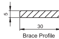
Brace Profile
