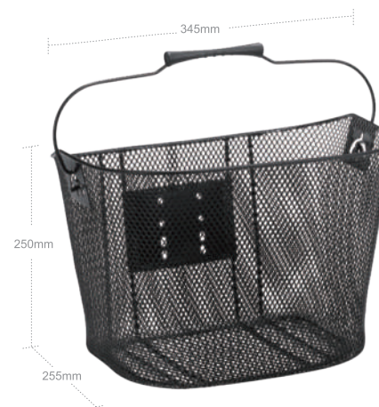
Upgraded Handle (BKG-11)
