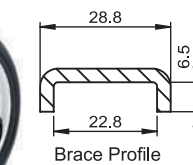
Brace Profile
