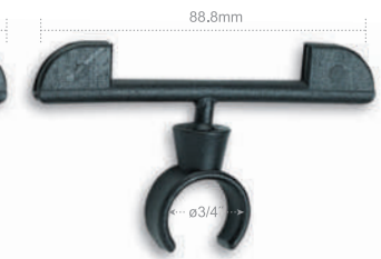
SW-412B Wider Price-card Holder (fit \phi 3/4" handlebar)
