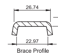
Brace Profile
