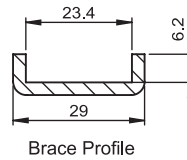
Brace Profile
