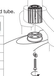
SB5-01 Exclusive Hardware
